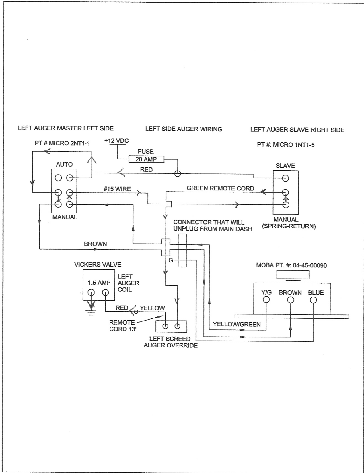
FIGURE 4-21. 8515, LEFT AUGER SWITCH WIRING
